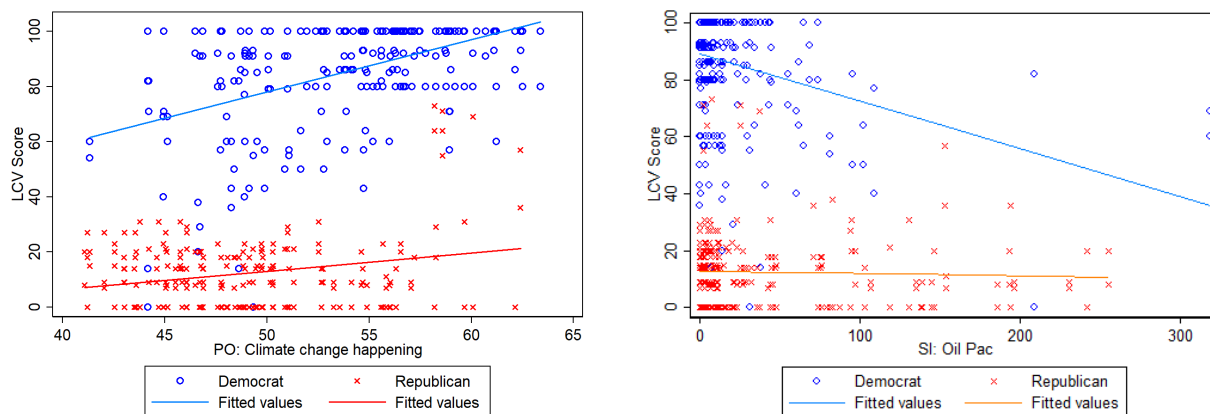
Figure 2: Scatterplot, LCV score on PO and Oil Contributions
