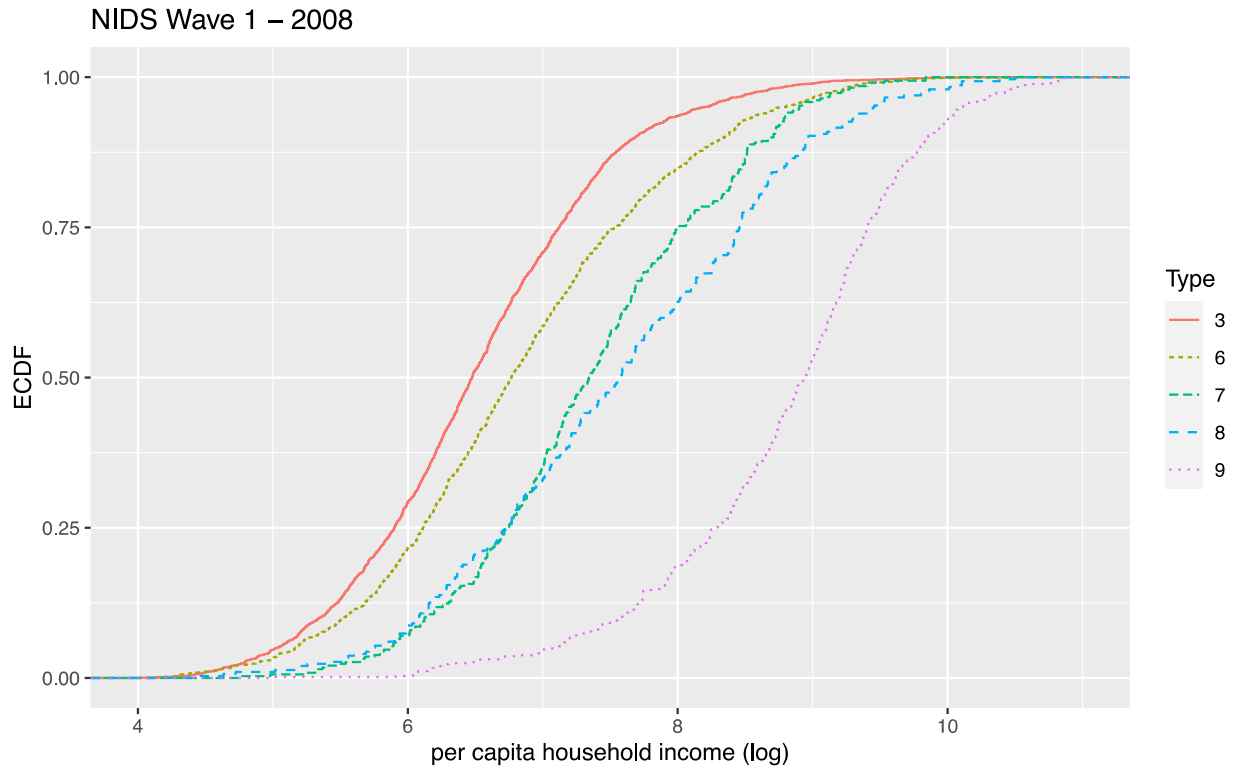
Figure 5: Empirical cumulative distribution functions for five types in South Africa: 2008
