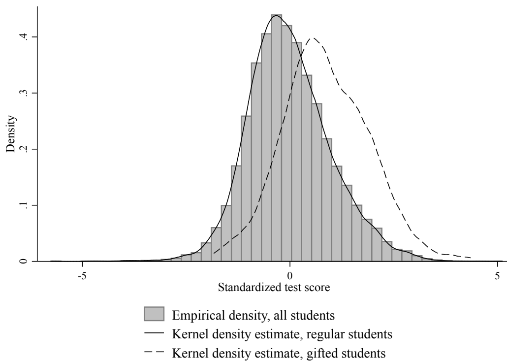
Figure 1: Distribution of test scores
