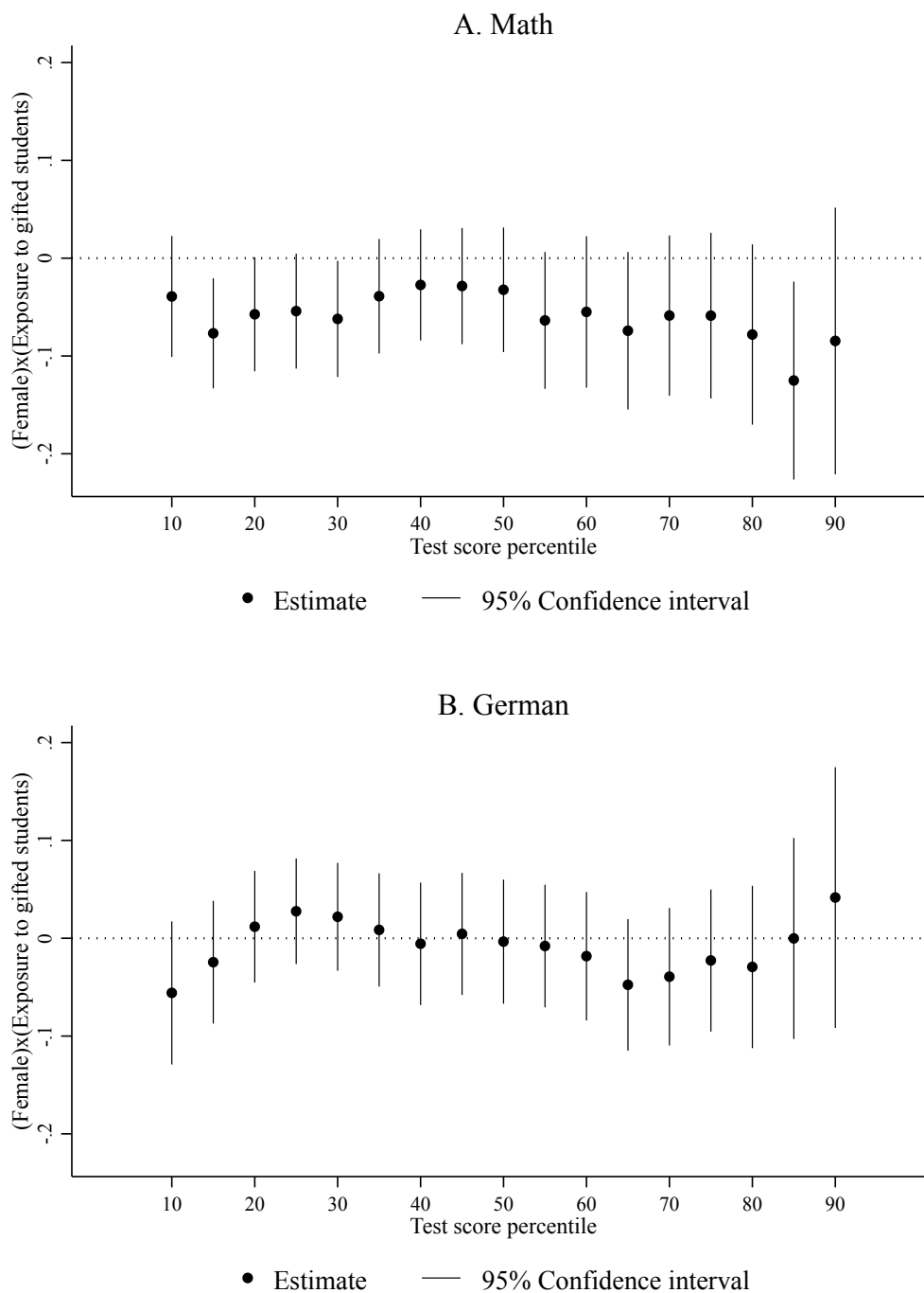
Figure A.8: Quantile treatment effect of exposure to gifted classmates for female students and male students
