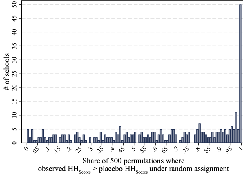
Figure C.1: The School-Level Concentration of Classrooms Based on Test Scores, With B = 400 Classroom Assignment Permutations
