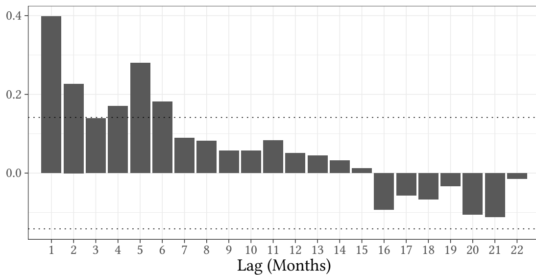
(b) Residual Autocorrelation Function
