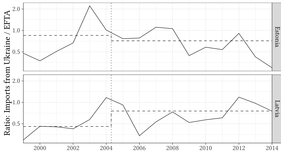
Trends in Import Penetration by Ukraine, Relative to EFTA
