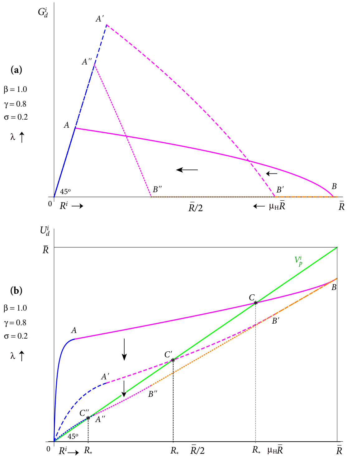
Figure B.2: Optimizing arming and payoffs under a unilateral deviation and various resource distributions: destruction
