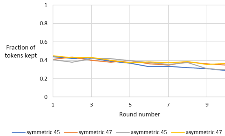
Figure 2b: Fraction of tokens kept
