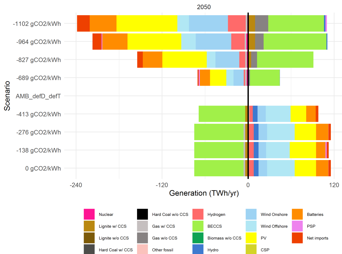
Figure 13. Change in generation in 2050 between BECCS emission factor scenarios and default AMB scenario ( -551 \text{ gCO}_2/\text{kWh}_{el} ) in the EU ETS. A positive value means there is higher generation in the corresponding scenario.
