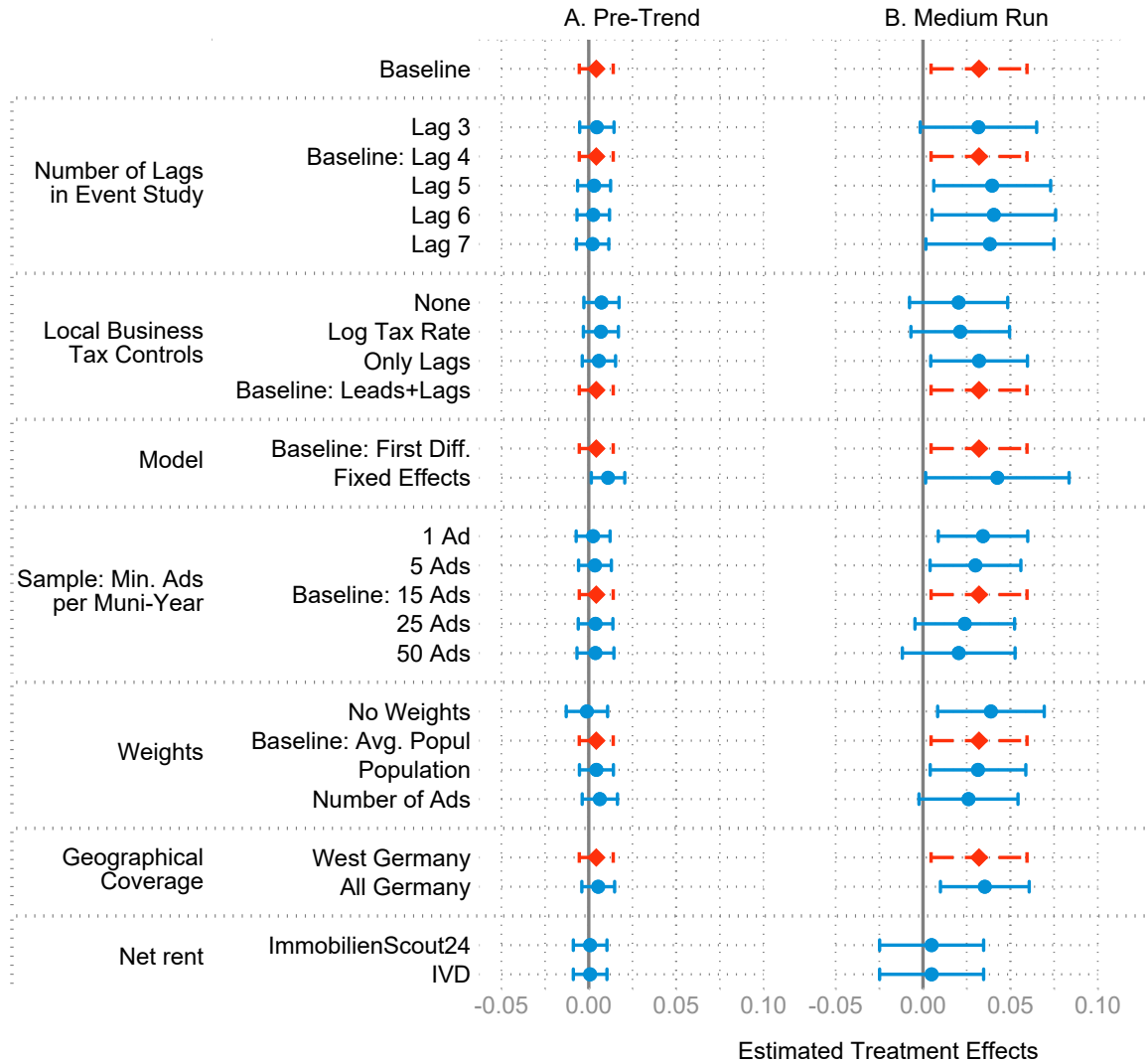
Figure 7: Robustness Checks
