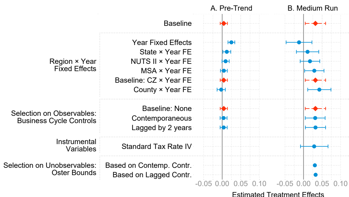
Figure 4: Probing Identification
