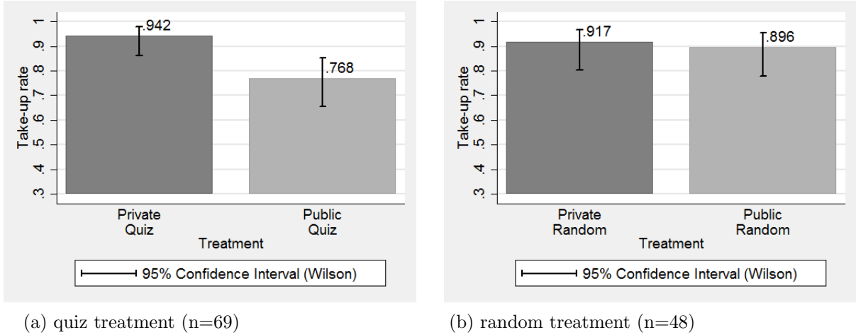
Figure 2: Take-up rate by transfer regime (subsidized treatments)
