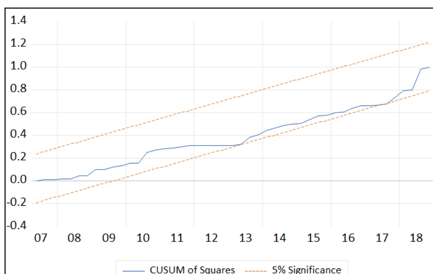
Graph of Cumulative sum of Squares
