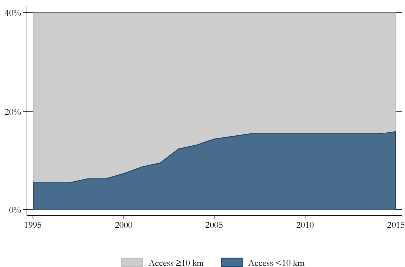
Figure 3.2: Sample balancedness
