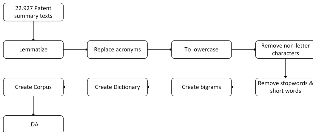
Figure 4: Data cleaning procedure
