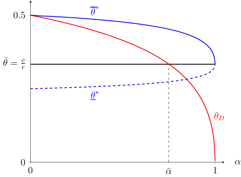
Figure 1: Equilibrium thresholds as a function of \alpha for r = 1 and c = w = \frac{1}{3} .
