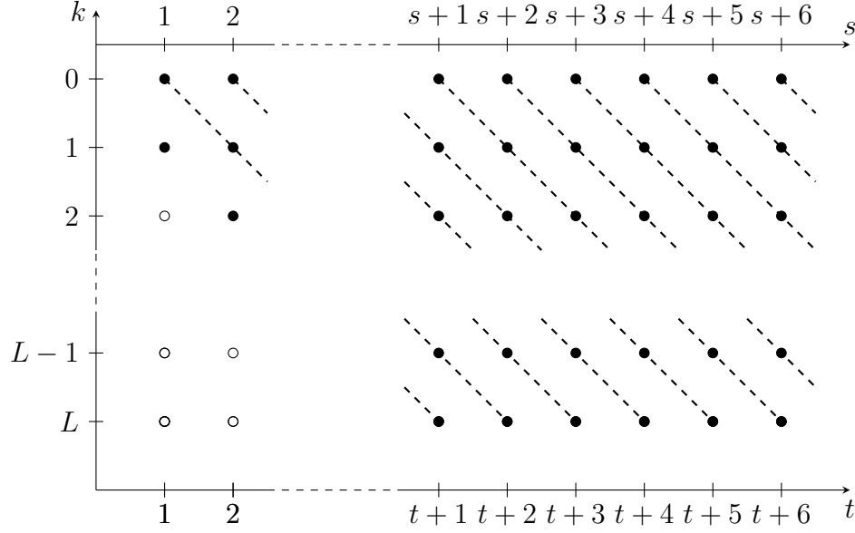
Figure C.1: Illustrating the re-indexing for the proof (the re-indexing omits k = L , since c_t(\ell^L) = c_\ell(F) is determined by Lemma B.7). The ladder- s resource constraints sum over the diagonal dashed lines, while the period- t resource constraints sum vertically. Since there is at most one realization of \ell in any history in period 1, k can only equal 0 or 1; similarly, in period 2, k \leq 2 .
