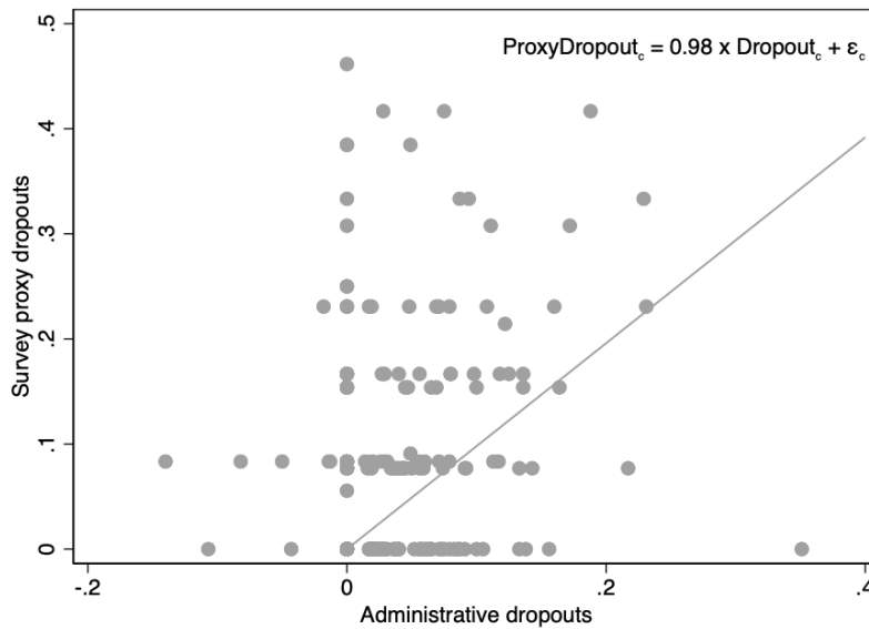
Figure B1. Binscatter plot of the survey proxy (averaged at the classroom level) and administrative data on student dropouts
