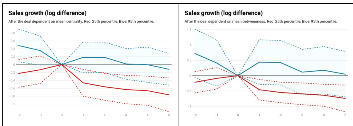
Figure 5: differences between high and low average centrality or betweenness of investors on the paths of growth of portfolio companies.
