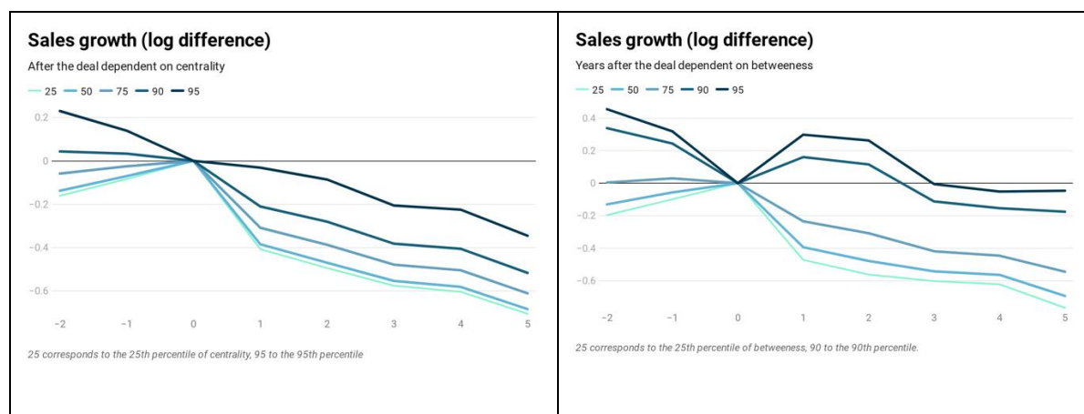
Figure 4: Sales growth after the deal dependent on maximum centrality (left panel) and betweenness (right panel)
