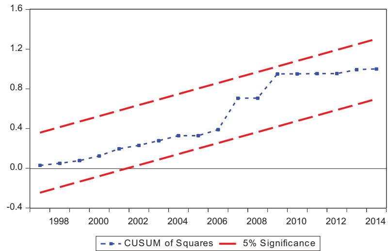
b. Plot of CUSUMSQ
