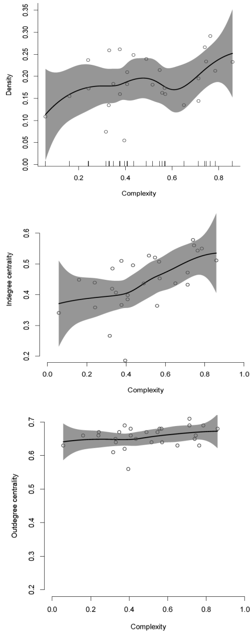
Figure 2: Relation between goods' complexity index and network indices
