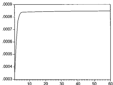
Response of NL_CPI_LOG to Cholesky One S.D. NLEFF_LOG_M Innovation
