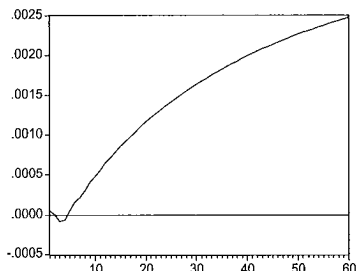
Response of FRA_CPI_LOG to Cholesky One S.D. FRAEFF_LOG_M Innovation
