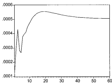
Response of GER_CPI_LOG to Cholesky One S.D. GEREFF_LOG_M Innovation
