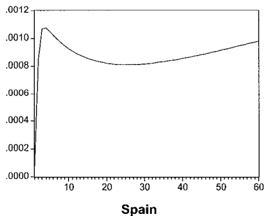
Response of SP_CPI_LOG to Cholesky One S.D. SPEFF_LOG_M Innovation
