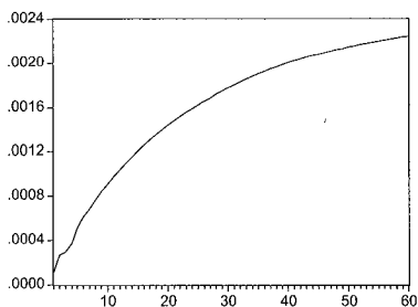
Response of IT_CPI_LOG to Cholesky One S.D. ITEFF_LOG_M Innovation
