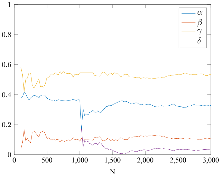
Figure 6.4: Example for estimations in a dynamically controlled survey.
