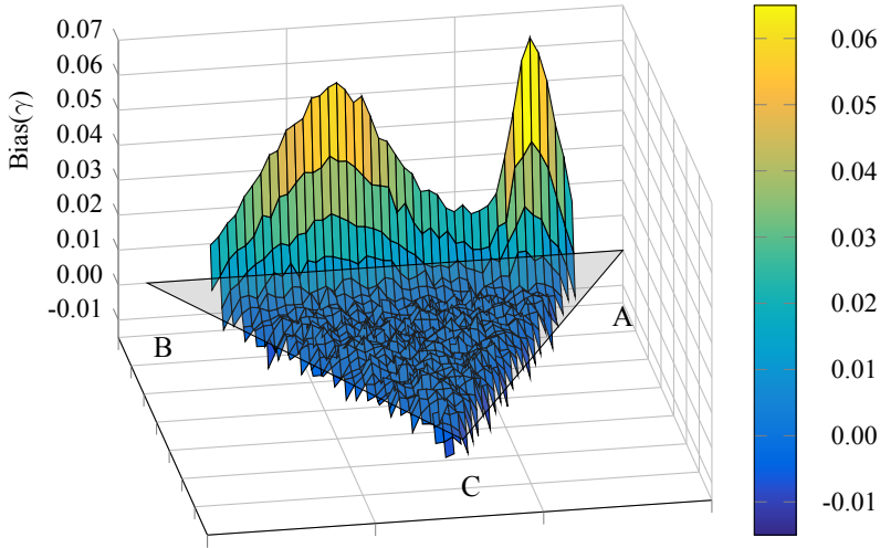
Figure 4.1: Estimation errors for \gamma in the TCD ( N = 1,500 , \delta = 0.20 , 1,000 repetitions).
