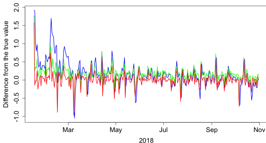
Figure 3: Difference between the true (30-day rolling volatility of CRIX) and the HAR, EWMA and LSTM models
