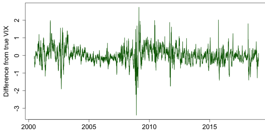
Figure 6: Difference between true and estimated VIX, values from 2000 to 2019. One can observe that the proposed model lags in catching the big spikes but performs well when market volatility is lower.
