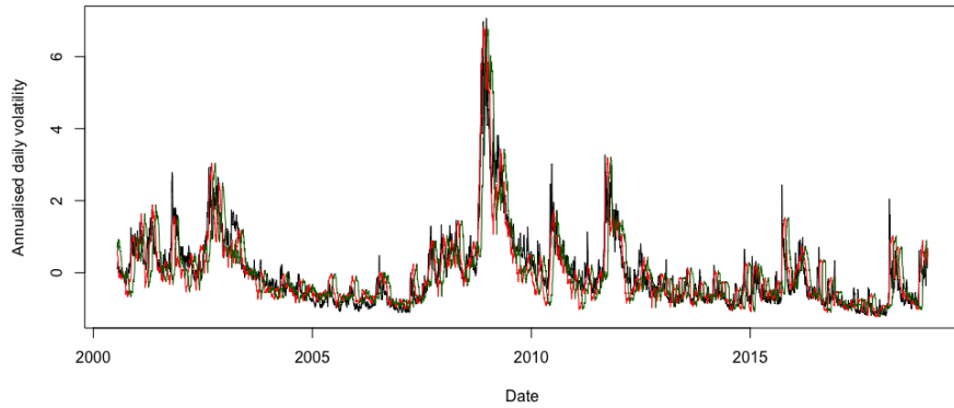
Figure 5: VIX estimated with HAR model on scaled daily volatility of SPY log-returns, VIX estimated with HAR with 21 days lag and true VIX values from 2000 to 2019
