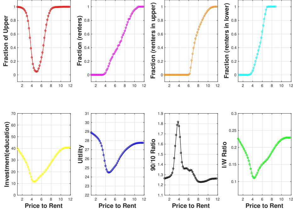
Figure 8: Bootstrapping Results
