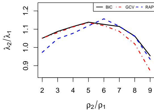
Figure 6: Relative changes of \lambda in dependence on relative changes of the covariance parameter \rho , for BIC (solid), GCV (dot-dashed) and RAP (dashed) method.
