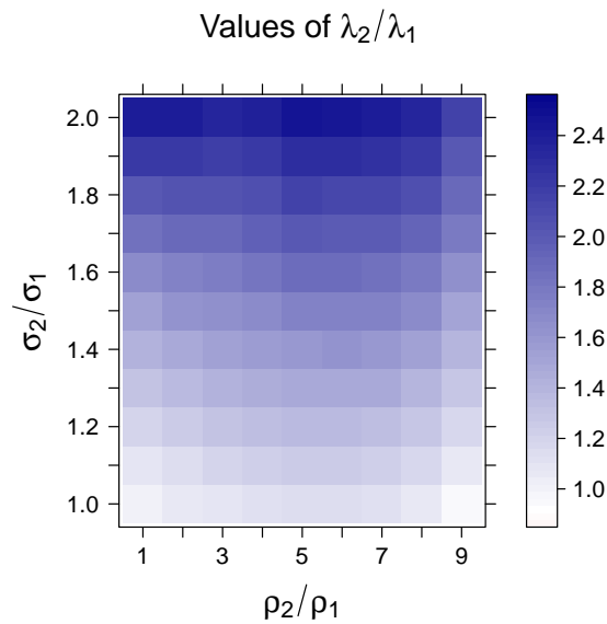
Figure 10: Relative changes of \lambda corresponding to the combination of relative changes of \rho and \sigma .
