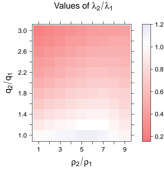
Figure 12: Relative changes of \lambda corresponding to the combination of relative changes of q and \rho .
