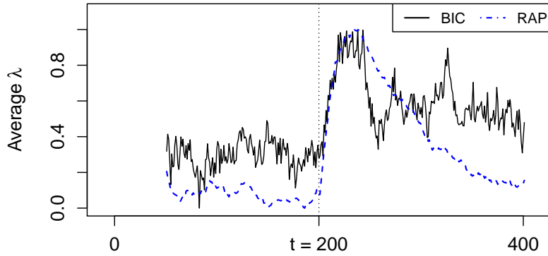
Figure 3: Standardized series of average \lambda over 100 scenarios with a change point at t_0 = 200 and \beta_{1,2} defined by (4), for BIC (solid) and RAP (dashed) method.
