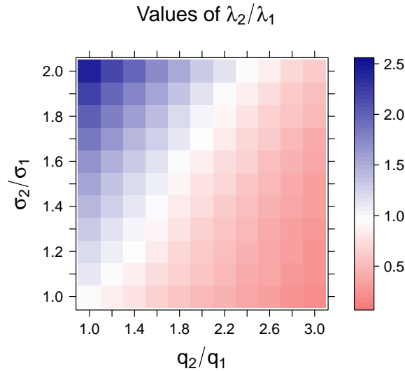
Figure 8: Relative changes of \lambda corresponding to the combination of relative changes of q and \sigma .
