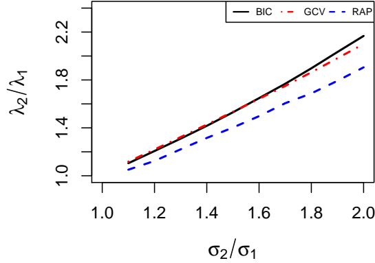
Figure 1: Relative changes of \lambda in dependence on relative changes of the standard deviation, \sigma , for BIC (solid), GCV (dot-dashed) and RAP (dashed) method.
