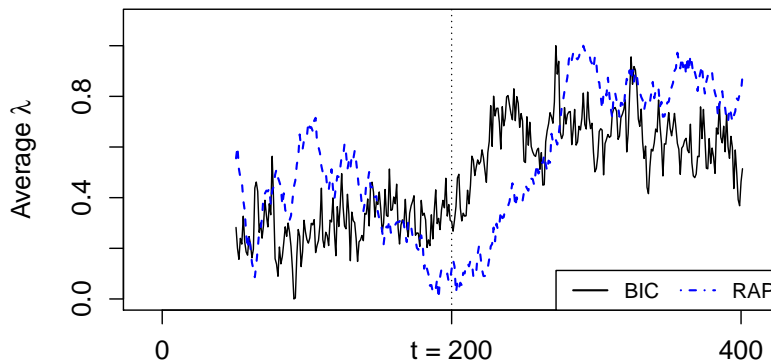
Figure 7: Standardized series of average \lambda over 100 scenarios with a change point at t_0 = 200 and \rho_1 = 0.1 and \rho_2 = 0.5 , for BIC (solid) and RAP (dashed) method.
