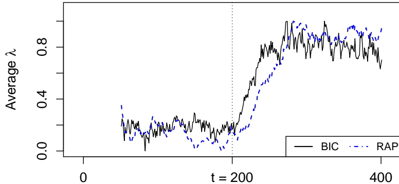
Figure 2: Standardized series of average \lambda over 100 scenarios with a change point at t_0 = 200 and \sigma_1 = 1 and \sigma_2 = 1.5 , for BIC (solid) and RAP (dashed) method.
