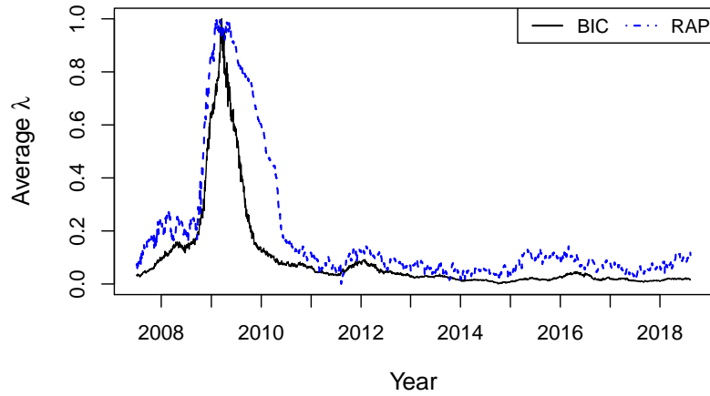
Figure 14: Standardized series of average \lambda in the US stock returns data, daily observations from January 3, 2007, to August 10, 2018, for BIC (solid) and RAP (dashed) method.
