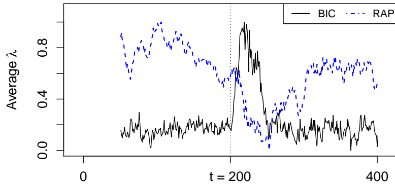
Figure 9: Standardized series of average \lambda over 100 scenarios with a change point at t_0 = 200 and q_1 = 5 , q_2 = 9 , \sigma_1 = 1 , \sigma_2 = 1.6 and \rho_1 = \rho_2 = 0.1 , for BIC (solid) and RAP (dashed) method.
