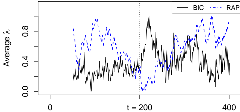
Figure 11: Standardized series of average \lambda over 100 scenarios with a change point at t_0 = 200 and \rho_1 = 0.1 , \rho_2 = 0.9 , \sigma_1 = 1 , \sigma_2 = 1.1 and q_1 = q_2 = 5 , for BIC (solid) and RAP (dashed) method.
