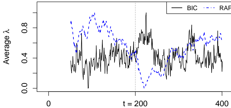
Figure 13: Standardized series of average \lambda over 100 scenarios with a change point at t_0 = 200 and q_1 = 5 , q_2 = 6 , \rho_1 = 0.1 , \rho_2 = 0.4 and \sigma_1 = \sigma_2 = 1 , for BIC (solid) and RAP (dashed) method.
