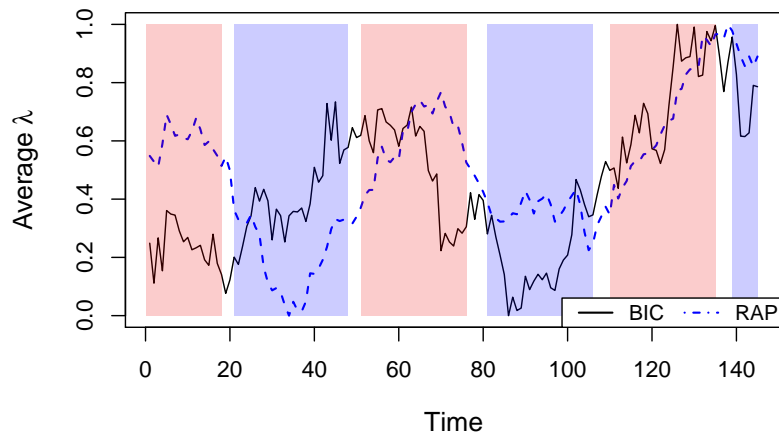
Figure 15: Standardized series of average \lambda in the fMRI dataset, for BIC (solid) and RAP (dashed) method. Distinct tasks are indicated by the background colour (red indicates a neutral task, blue indicates an emotion task and white denotes the resting period).
