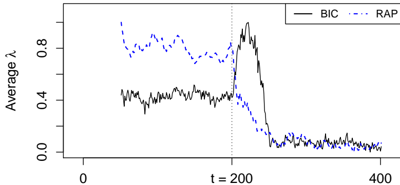
Figure 5: Standardized series of average \lambda over 100 scenarios with a change point at t_0 = 200 and q_1 = 5 and q_2 = 10 , for BIC (solid) and RAP (dashed) method.
