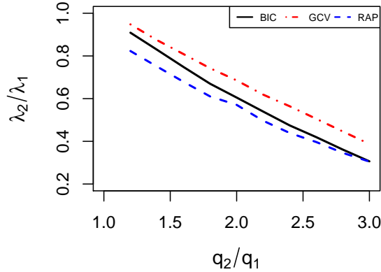
Figure 4: Relative changes of \lambda in dependence on relative changes of the size of the active set q , for BIC (solid), GCV (dot-dashed) and RAP (dashed) method.
