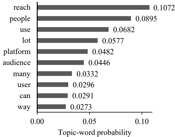
Figure 6. Topic-word probabilities for the exemplary topic B (LDA).
