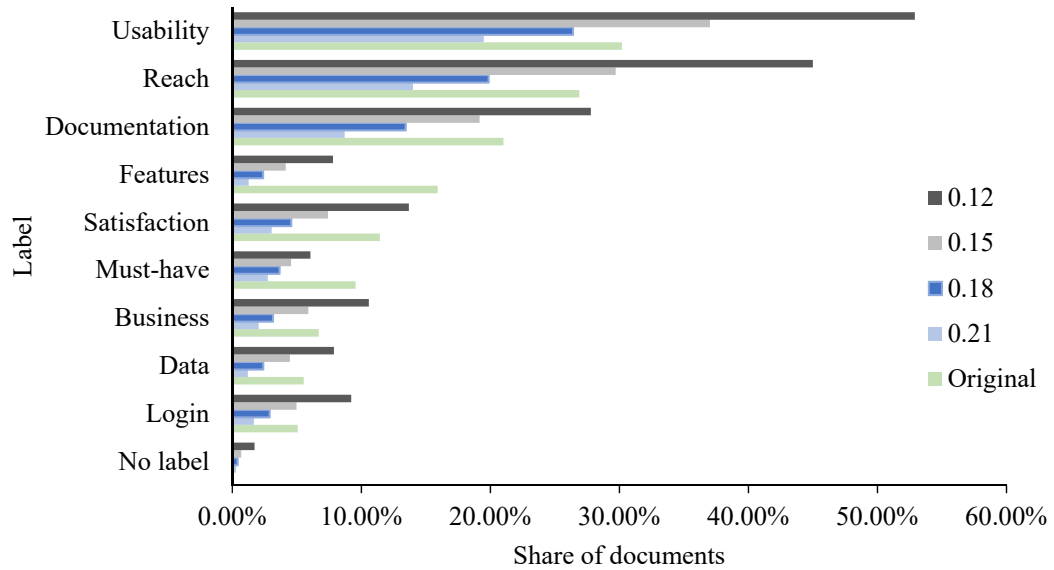
Figure 10. WNTM topic distribution with different thresholds. Ordered by original share of labels.
