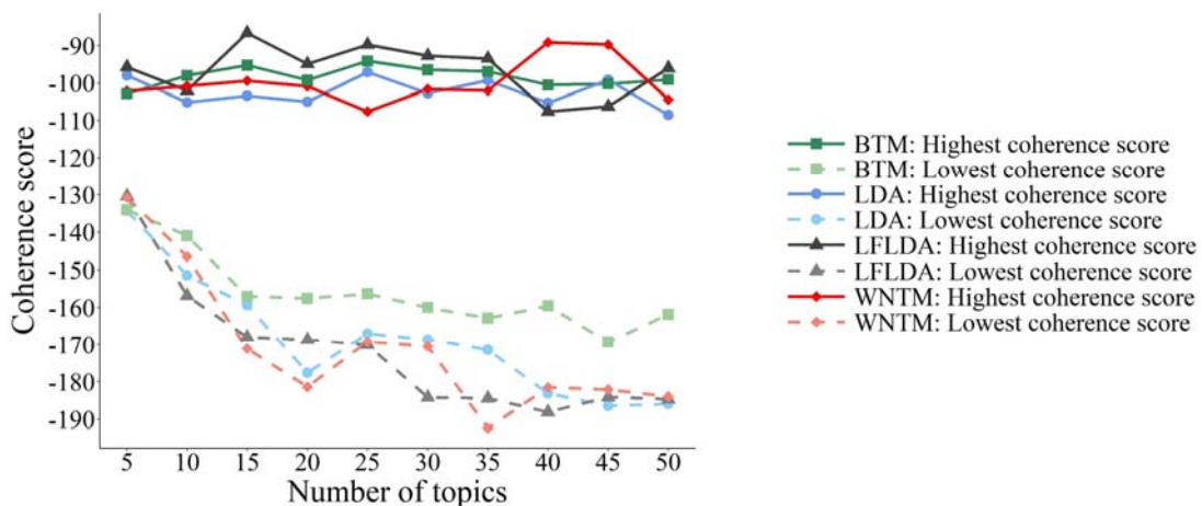
Figure 5. Highest and lowest coherence scores per method on the topic-level.
