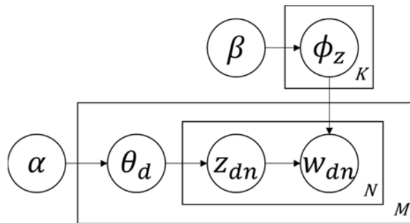
Figure 1. Graphical representation of the generative process of LDA. Adapted from [16, 28].
