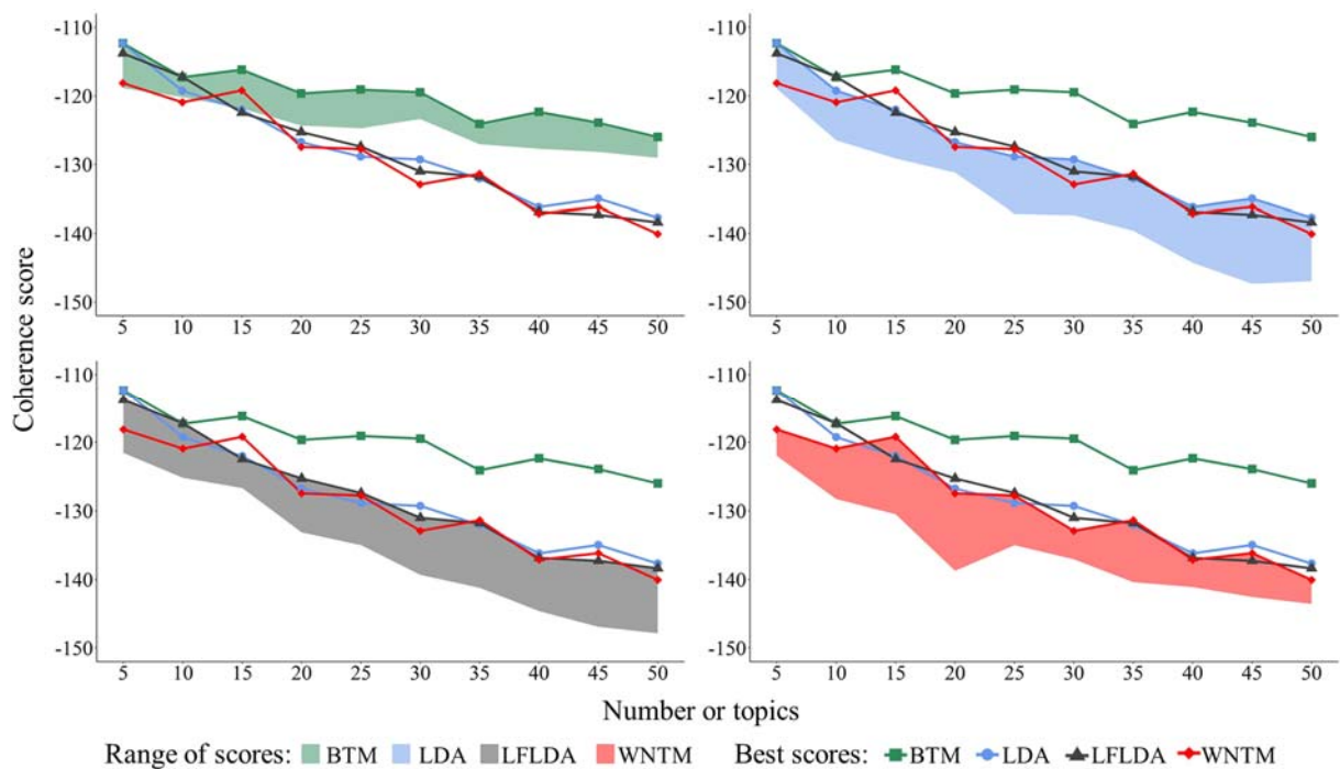
Figure 4. Best average coherence scores per method (lines) and range of average coherence scores per method produced by different hyperparameter combinations (shaded area).
