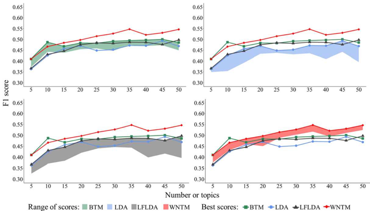
Figure 8. Best F1 score per method averaged over all labels (lines) and range of average F1 scores per method produced by different hyperparameter combinations (shaded area).
