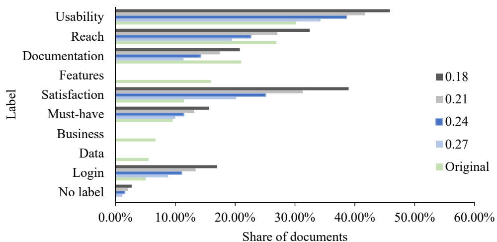
Figure 9. BTM topic distribution with different thresholds. Ordered by original share of labels.
