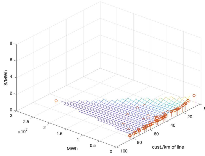
Figure A.2: Average cost curve for O&M costs (2009)
