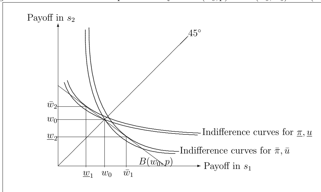
Figure 2: Illustration of the Unpredictability Set W(w_0, p) when (w_0, w_0) \in W(w_0, p)
