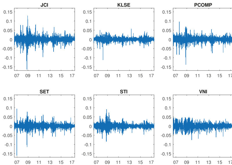
Figure 1. Log-returns for the period 1 July 2006–30 June 2017.
