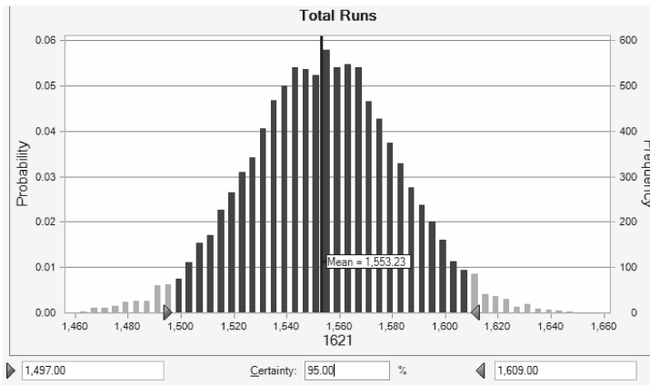
Figure 1. Monte Carlo Simulation for Number of Runs Observed over 10,000 Trials. This graph assumes the DSE based parameters of 3119 returns and a success rate of 53%.
