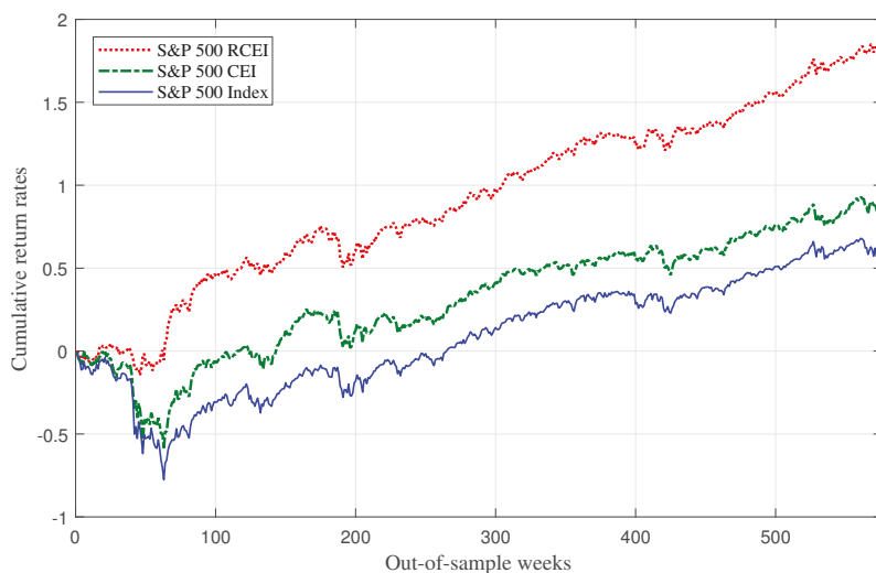
Figure 2. Out-of-sample performances of RCEI and CEI models in S&P 500.
