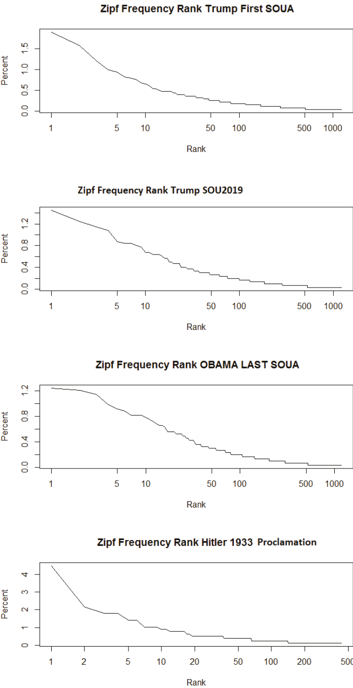
Figure 9. Zipf Plots.
