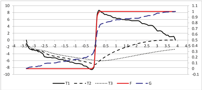
Figure 1. Ascending DD statistics distribution for C23-T33. Note: T_j is the test statistic defined in (3) for j = 1, 2 and 3. F and G are the CDFs of the excess warrant returns for C23 and T33, respectively.
