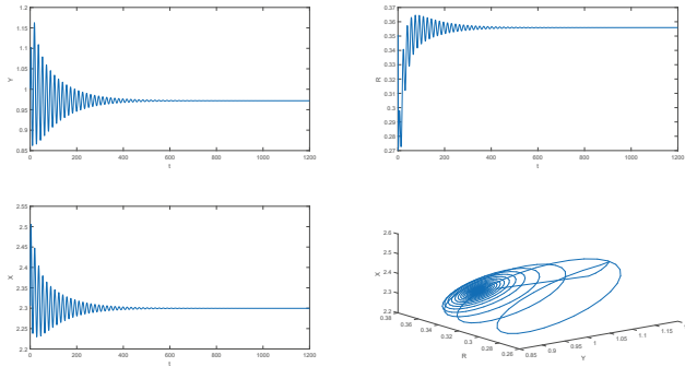
Figure 1. E^* is asymptotically stable, when \alpha = 0.98 , \tau = 3 .
