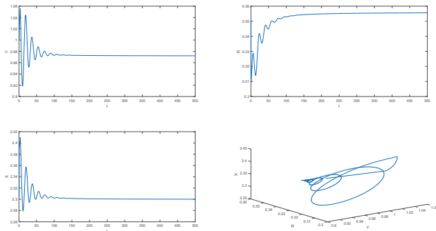
Figure 3. E^* is asymptotically stable, when \alpha = 0.9 , \tau = 3.2 .
