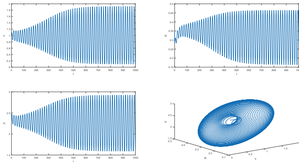
Figure 2. Stable periodic orbit of System (28), when \alpha = 0.98 , \tau = 3.2 .
