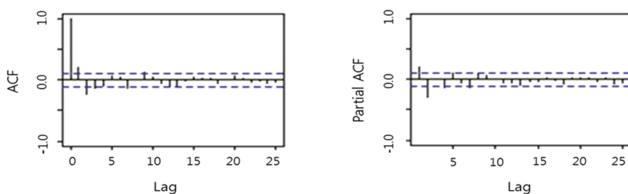
Figure 4. Plots of the autocorrelation function (ACF) and the partial autocorrelation function (PACF) of residuals.
