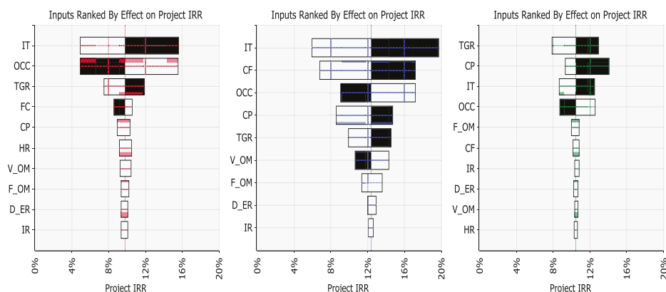
Figure 8. Project IRR tornado diagrams of Coal, Wind, and Nuclear.
