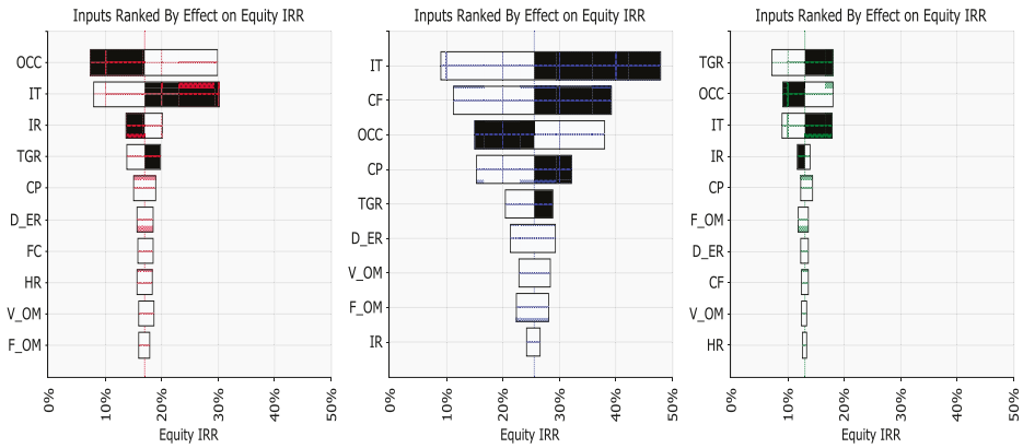
Figure 7. Equity IRR tornado diagrams of Coal, Wind, and Nuclear.
