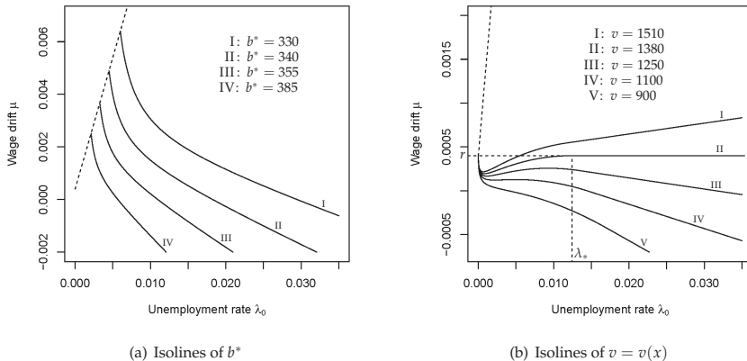
Figure 6. Isolines (level curves) of the optimal stopping problem solution on the (\lambda_0, \mu) -plane: (a) b^*(\lambda_0, \mu) = \text{const} (optimal threshold (23)); (b) v(\lambda_0, \mu) = \text{const} (value function (25)). The values of other parameters used throughout are as in Example 3: r = 0.0004 , P = 9000 , \beta = 30 , \sigma = 0.02 , and x = 346 . The slanted dashed lines in both plots show the boundary b^* = \lambda_0 + r (see (11)). In plot b, the horizontal dashed line indicates \mu = r and the vertical dashed line shows \lambda_* \doteq 0.012420 (cf. Figure 5b).
