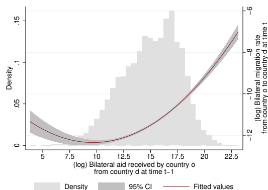
Figure A.1: Bilateral migration rates and bilateral aid
