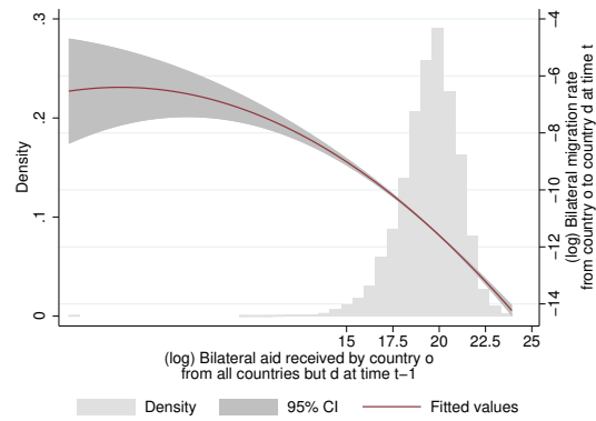
Figure A.2: Bilateral migration rates and remaining bilateral aid
