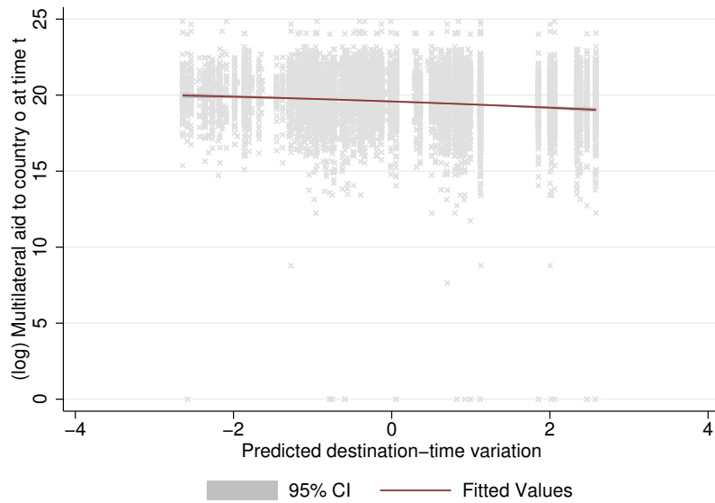
Figure A.4: Correlation between destination-time variations in migration rates and multilateral aid flows
