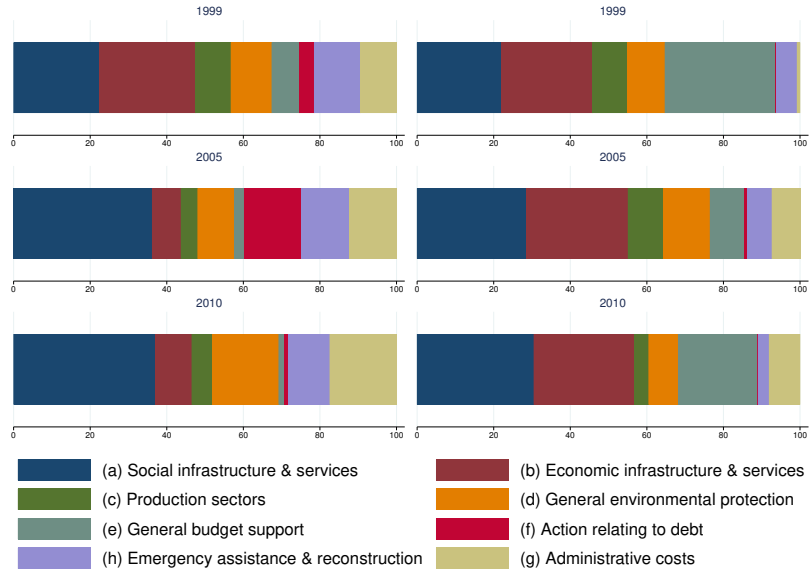
Figure A.6: Distribution of total bilateral and multilateral aid across sectors from 1999 to 2010
