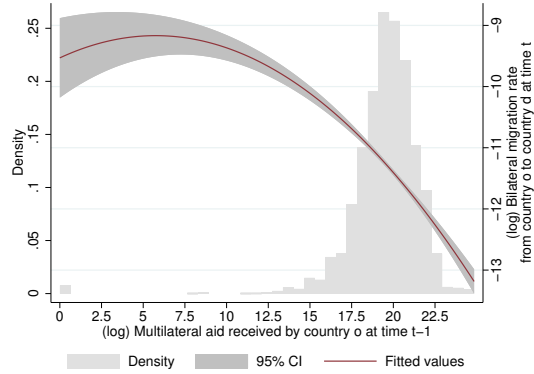
Figure A.3: Bilateral migration rates and multilateral aid
