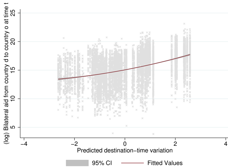
Figure A.5: Correlation between destination-time variations in migration rates and bilateral aid flows
