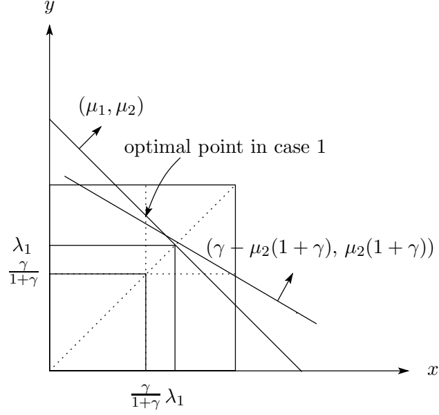
Figure 7: Optimal choice of (x, y) in case 1
