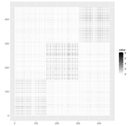
Figure 3: WF-SOFAR estimate
