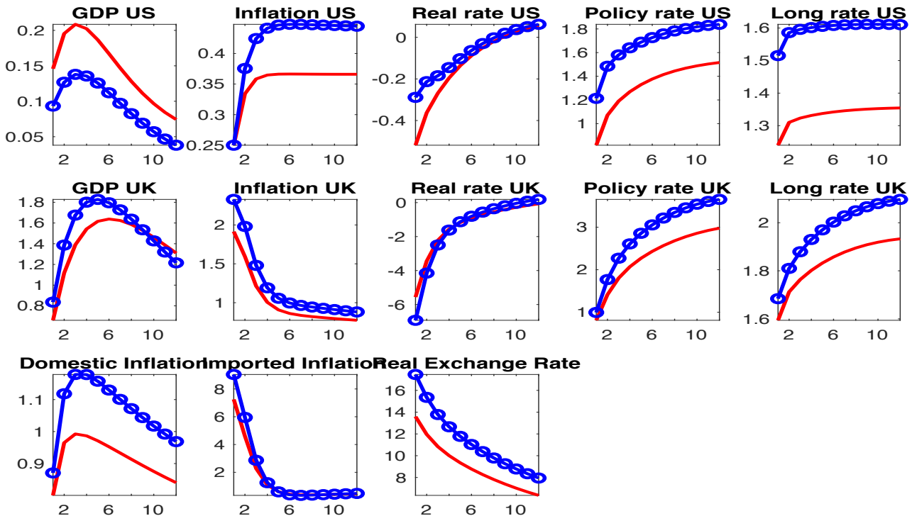
Figure 2: US Inflation Target Shock
