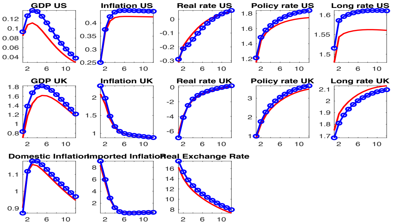
Figure 6: US Inflation Target Shock
