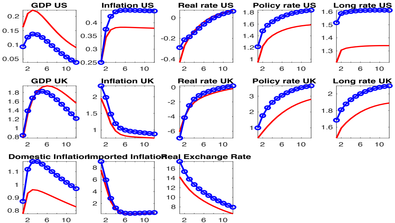
Figure 4: US Inflation Target Shock
