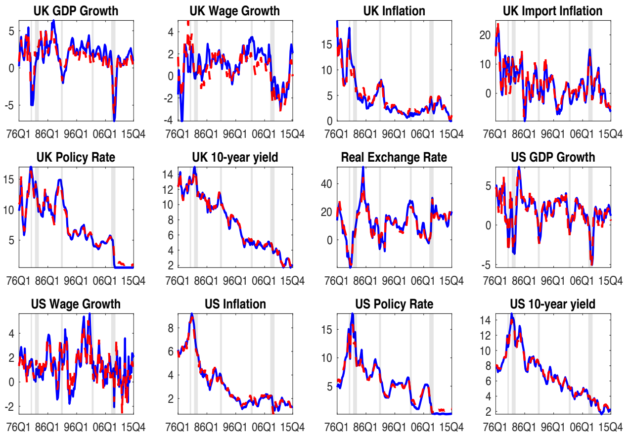
Figure 9: DSGE Model Fit
