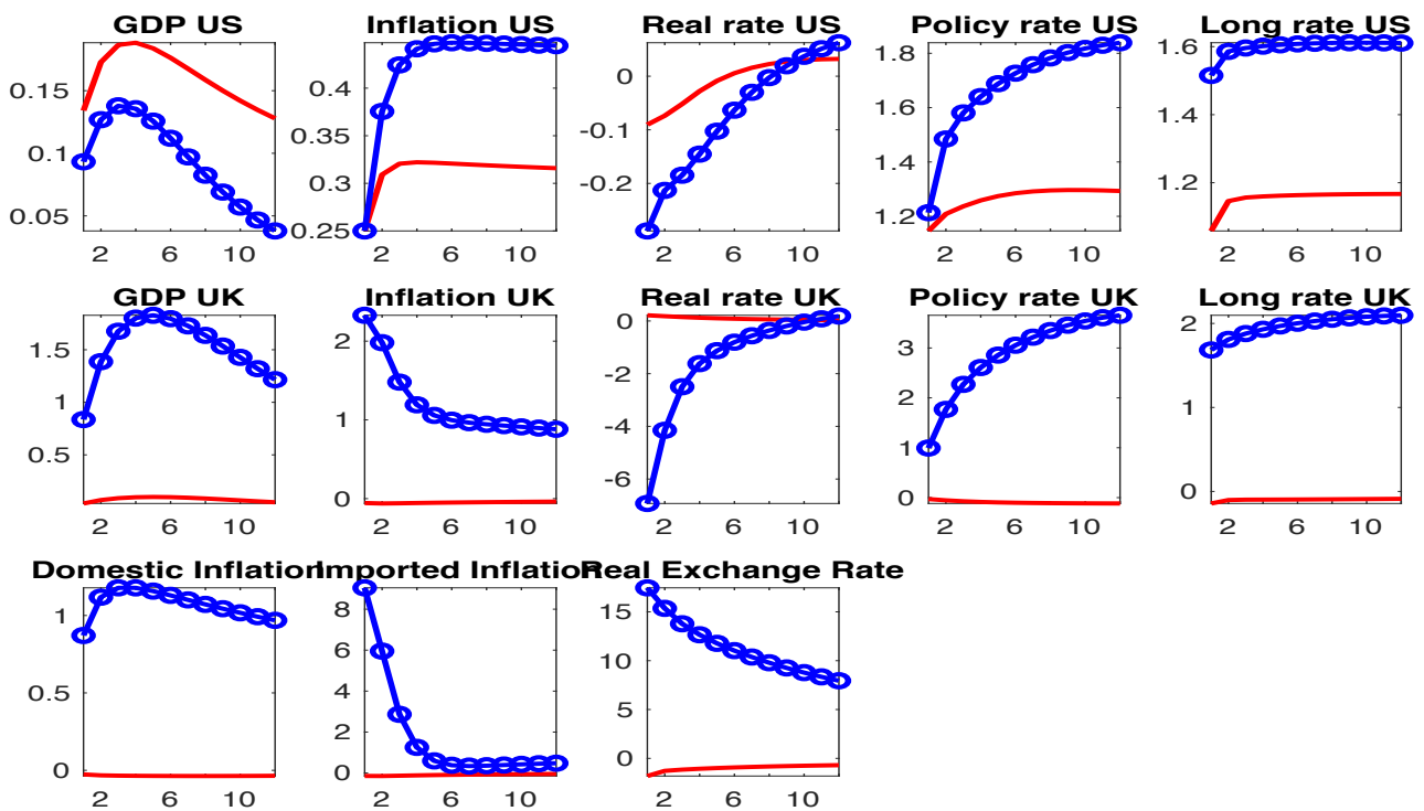
Figure 10: US Inflation Target Shock
