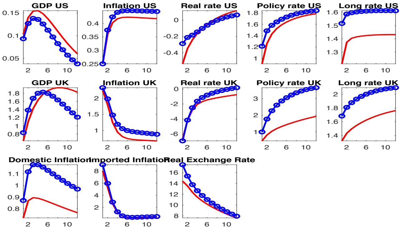
Figure 8: US Inflation Target Shock
