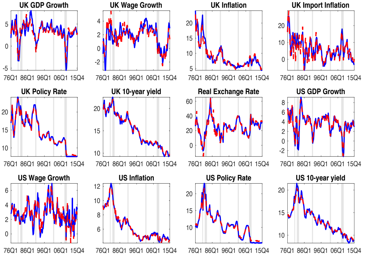
Figure 7: DSGE Model Fit
