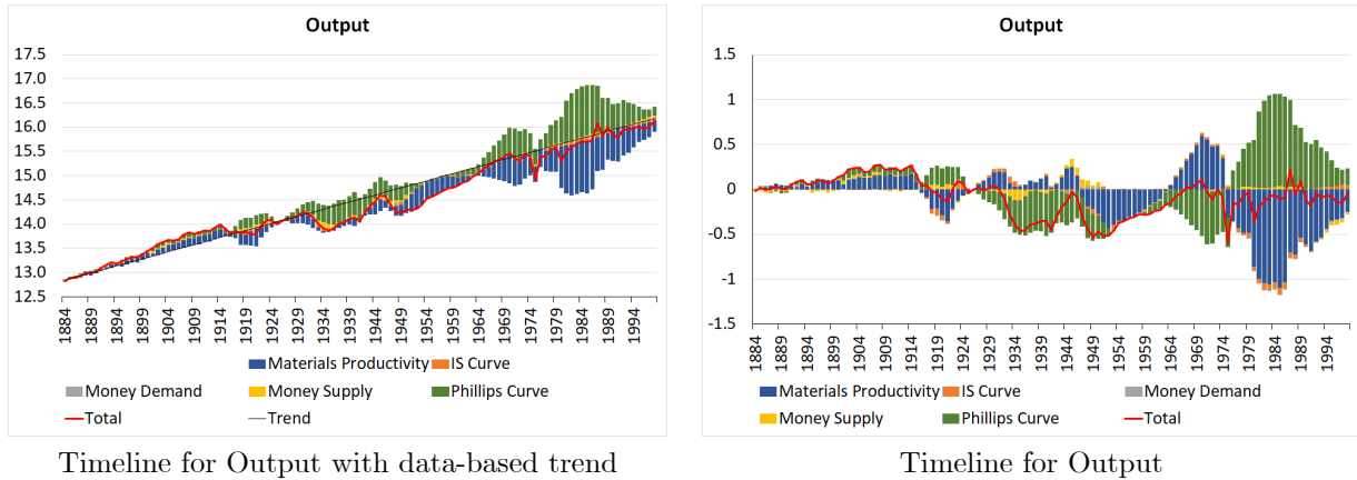
Figure 10: Timelines for Output
