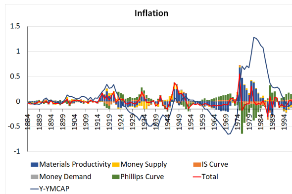
Figure 11: Timeline for Inflation
