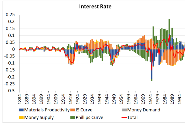
Figure 12: Timeline for Interest Rate
