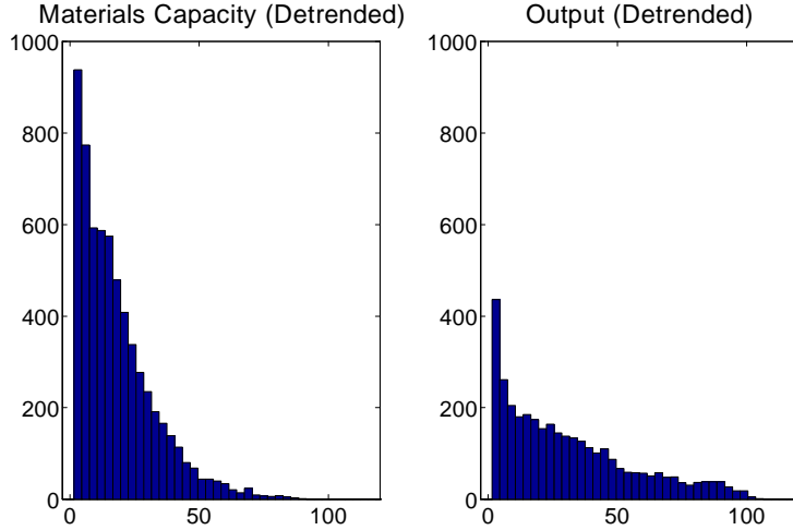
Figure 13: Histograms of Cycle Lengths
