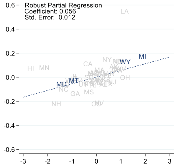
FIGURE 7. ROBUST PARTIAL REGRESSION PLOTS FROM MODEL OF STATE SPACE MODEL PERFORMANCE
