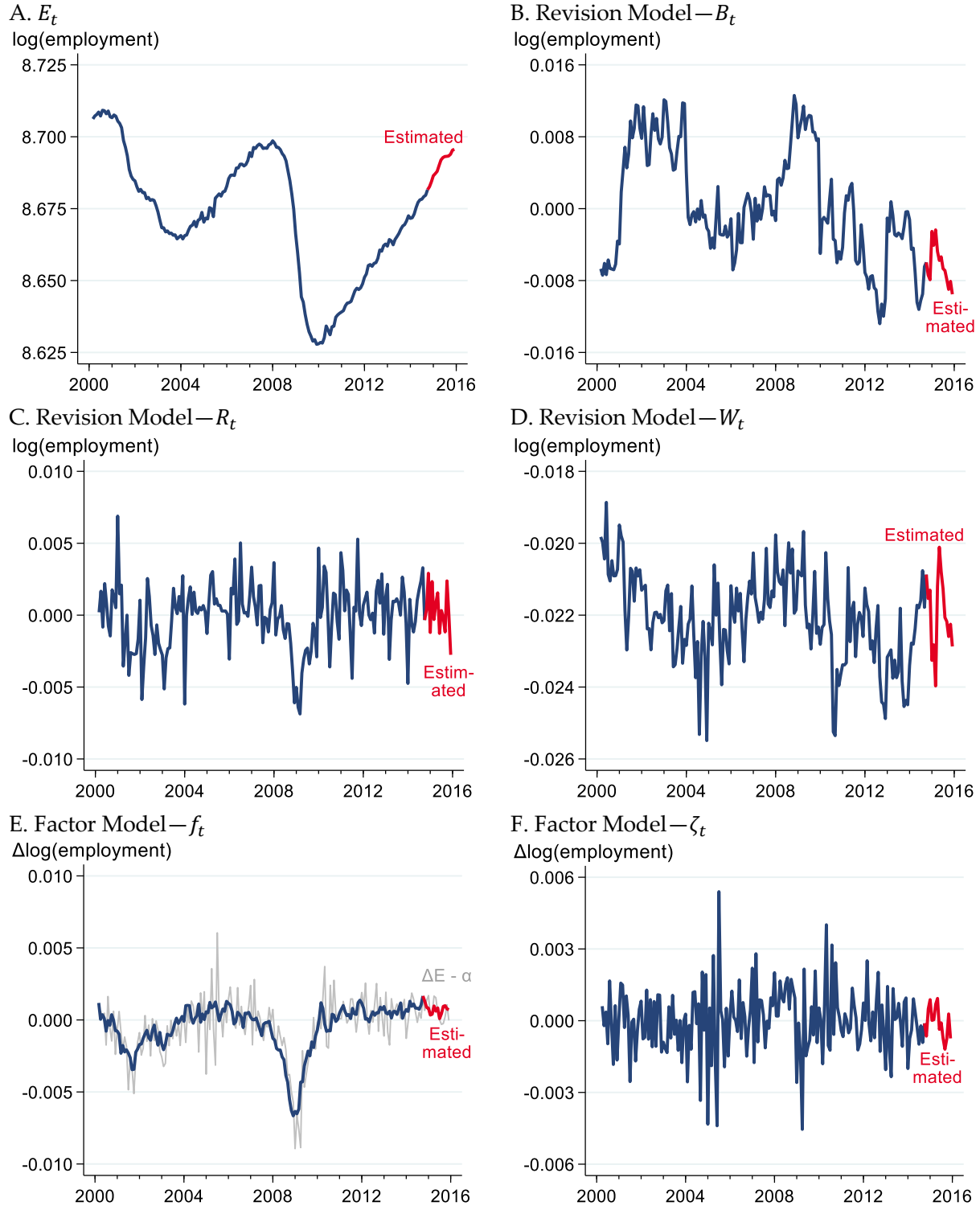
FIGURE 5. UNOBSERVED COMPONENTS FOR THE ILLINOIS JANUARY 2016 VINTAGE
