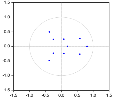
Stability test for inflation model (VAR)
