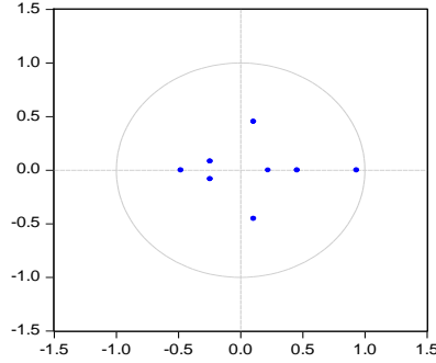
Stability test for inflation model (SW)
