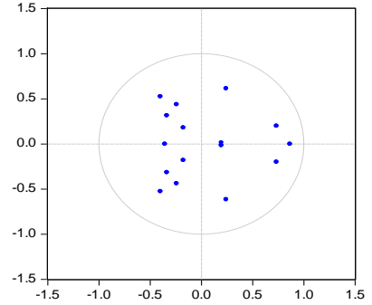
Stability test for inflation model (FAVAR)
