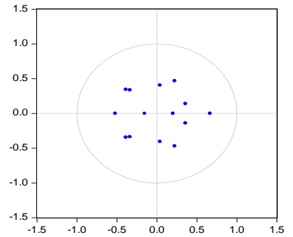
Stability test for output model (FAVAR)
