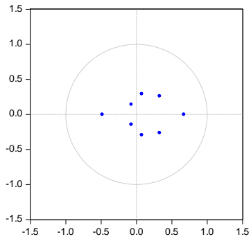
Stability test for output model (VAR)
