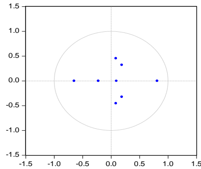
Stability test for output model (SW)
