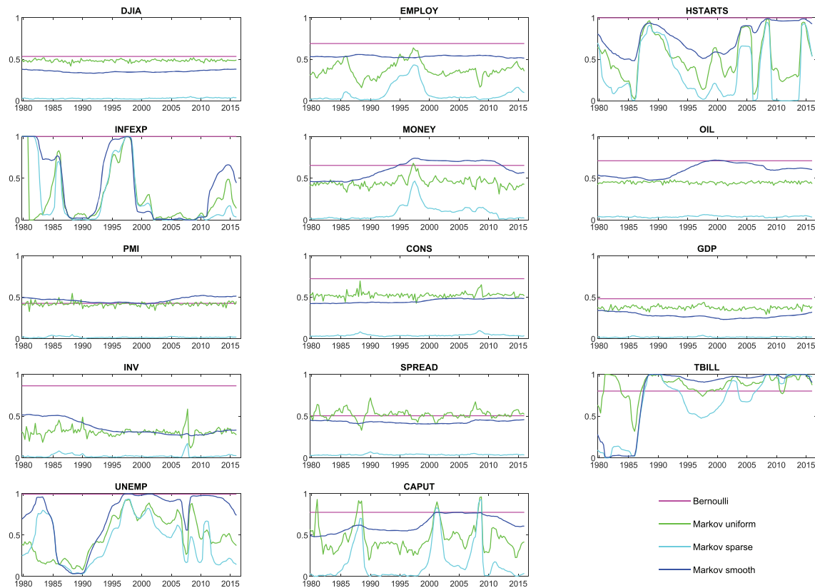
FIGURE C2 Variable inclusion probabilities for one-year PCE-deflator inflation [Colour figure can be viewed at wileyonlinelibrary.com ]
