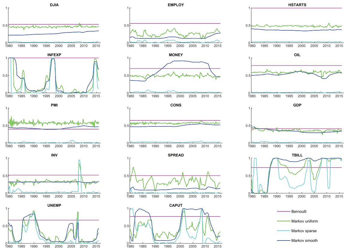
FIGURE C6 Variable inclusion probabilities for one-year CPI inflation [Colour figure can be viewed at wileyonlinelibrary.com ]
