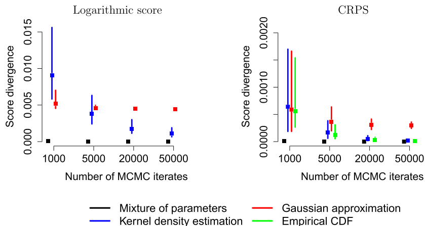
Figure 1. Score divergences in the simulation study with (\alpha, s, n) = (0.5, 2, 12) . For a given method and Markov chain Monte Carlo (MCMC) sample size, the bars range from the 10th to the 90th percentile of the score divergences across 1 000 replicates. The squares mark the respective medians. CDF, cumulative distribution function; CRPS, continuous ranked probability score.
