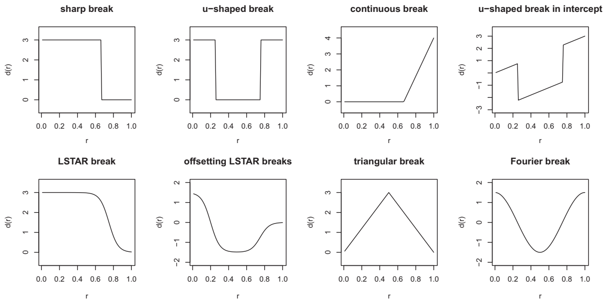
Figure 1. Plots of the trend functions. Note: The plots of the of the trend functions from Table II are presented. The trend size is \lambda = 3
