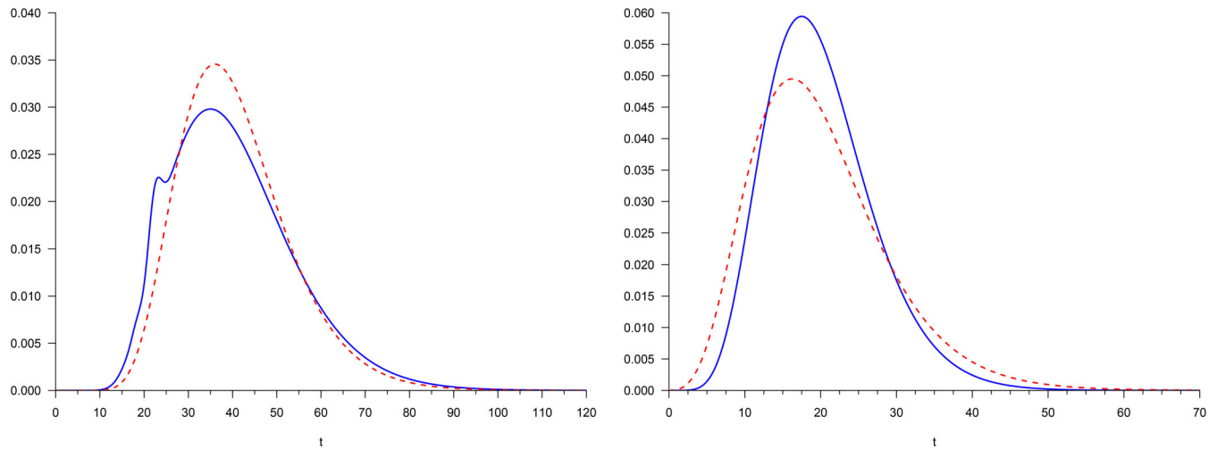
FIGURE 3 Plots of density functions f_{\hat{\theta}_0} (left) and f_{\hat{\theta}_0, \hat{\theta}_1} (right) and for Type-M (solid blue line) and Type-P (dashed red line) with true values \theta_0 = 40 and \theta_1 = 20 (see caption of Table 1) [Colour figure can be viewed at wileyonlinelibrary.com]
