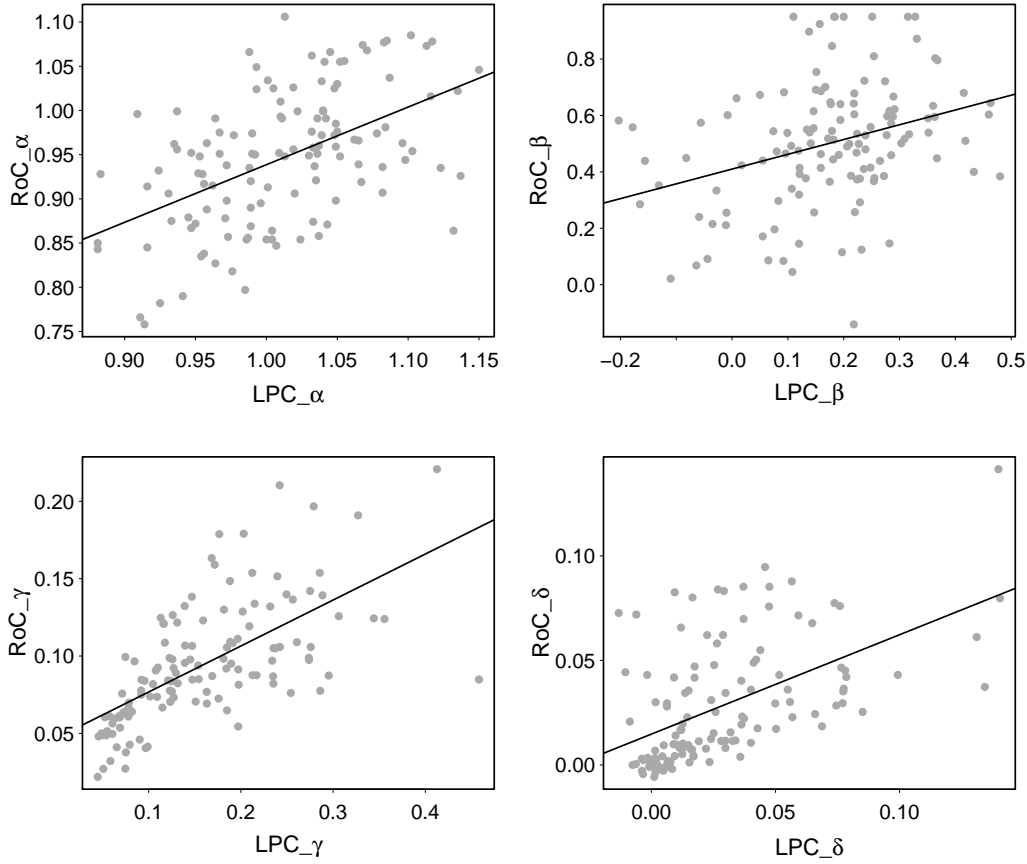
Figure 9: Scatter plot of Lévy parameters of Returns on Capital ( ROC ) and Labor Productivity Change ( \Delta LP ). All four parameters tend to be positively correlated.
