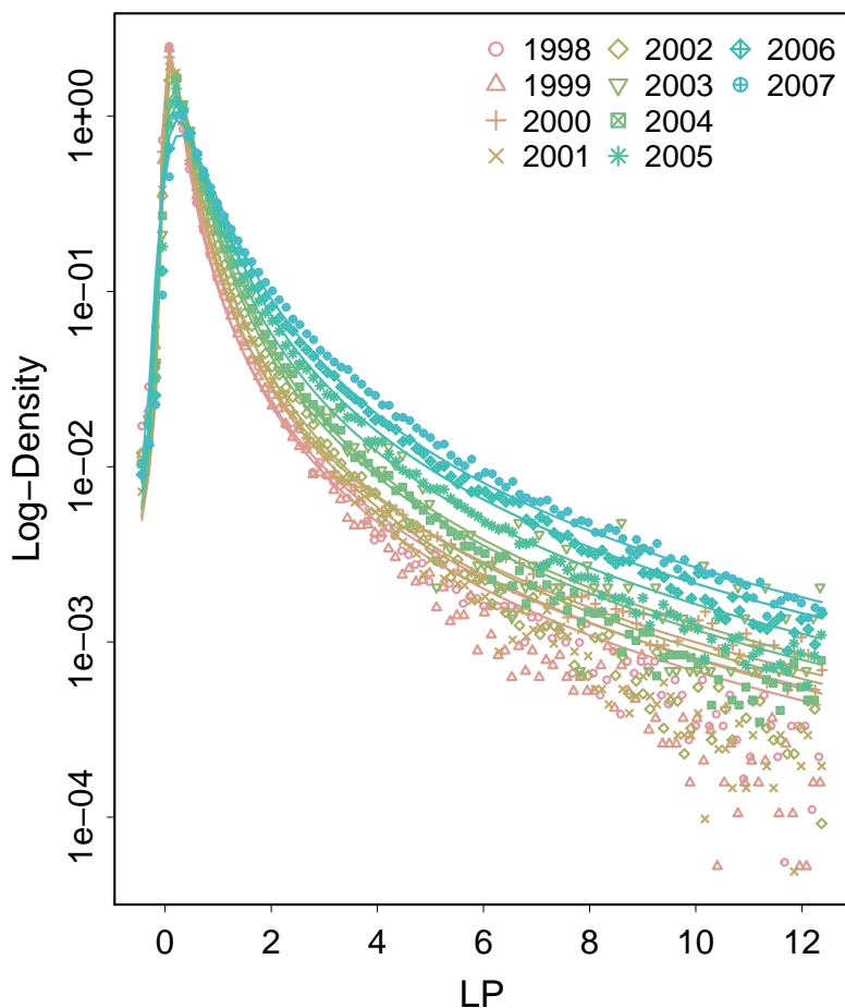
Figure 1: Density of the labor productivity ( LP ) distribution (full sample) by year in semi-log (vertical axis logarithmic). Solid lines indicate Levy alpha stable distribution fits as reported in Table 2.
