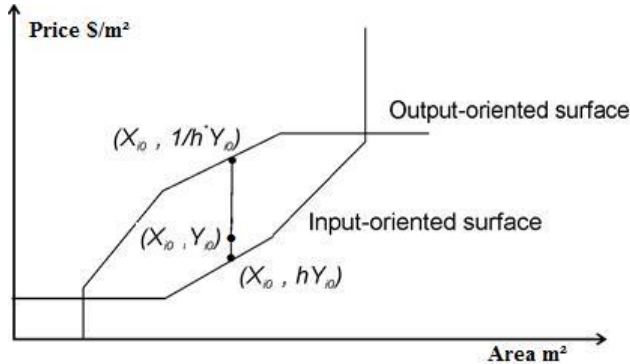
Figure 12. DP-DEA Buyer and Seller Perspective Surfaces
