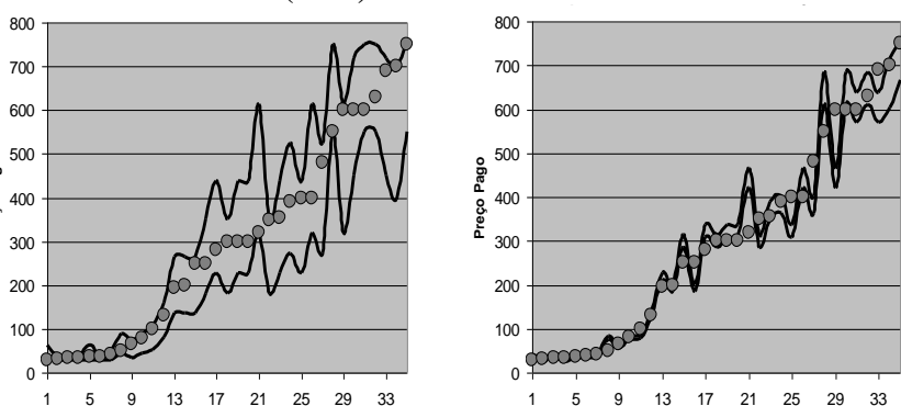
Figure 7. Comparing DP-DEA Buyer and Seller Surfaces fitness with L.R. Confidence Interval (80%)
