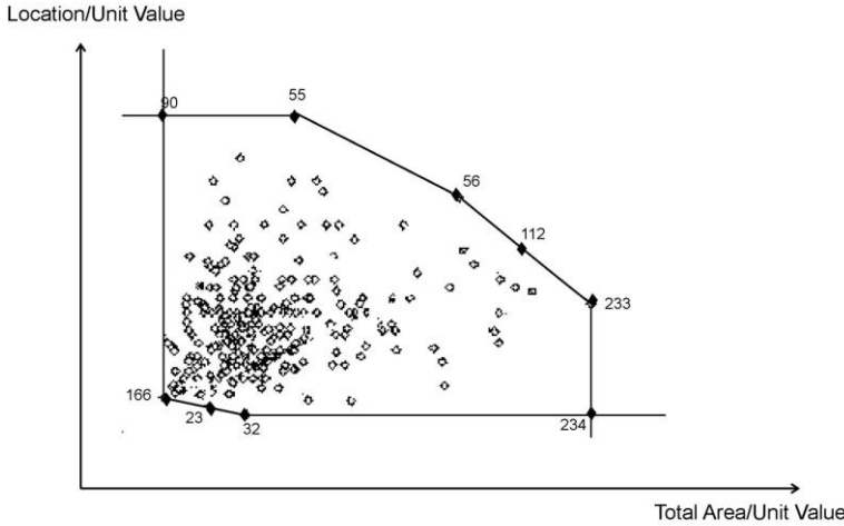
Figure 5. DP-DEA Envelopment Surfaces – Seller and Buyer Perspectives
