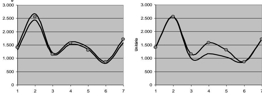
Figure 6. Comparing L.R. Confidence Interval (80%) fitness with DP-DEA Buyer and Seller Surfaces
