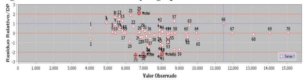
Figure 27. Outliers and errors analysis graph
