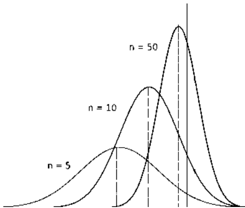
Figure 16. Consistency
