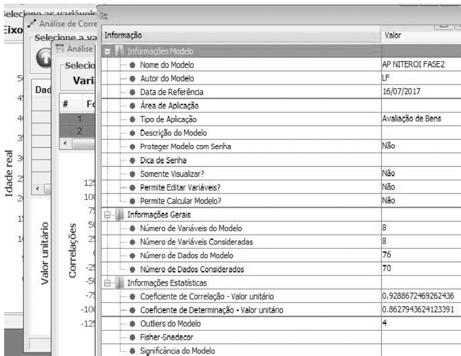
Figure 31. R 2
