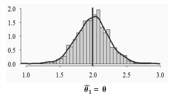
Figure 14. No tendency
