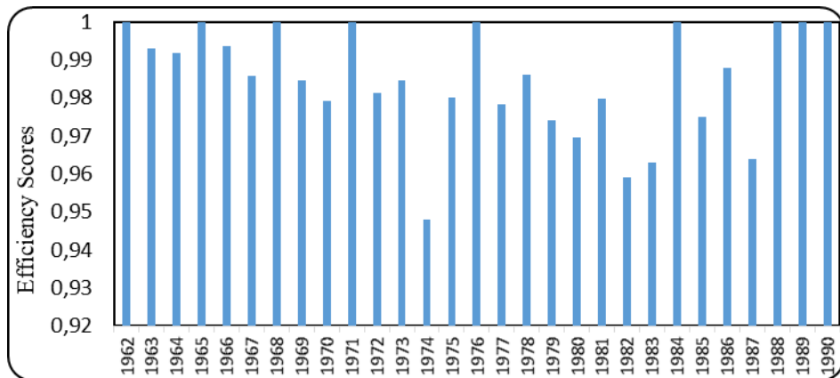
Figure 1. VRS efficiency: 1962-1990
