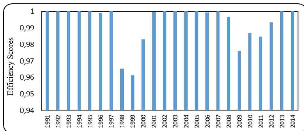
Figure 2. VRS efficiency: 1991-2014
