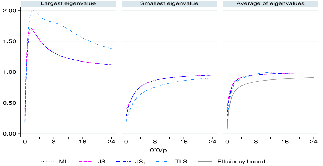
Figure 2: James–Stein class eigenvalues for p = 5
