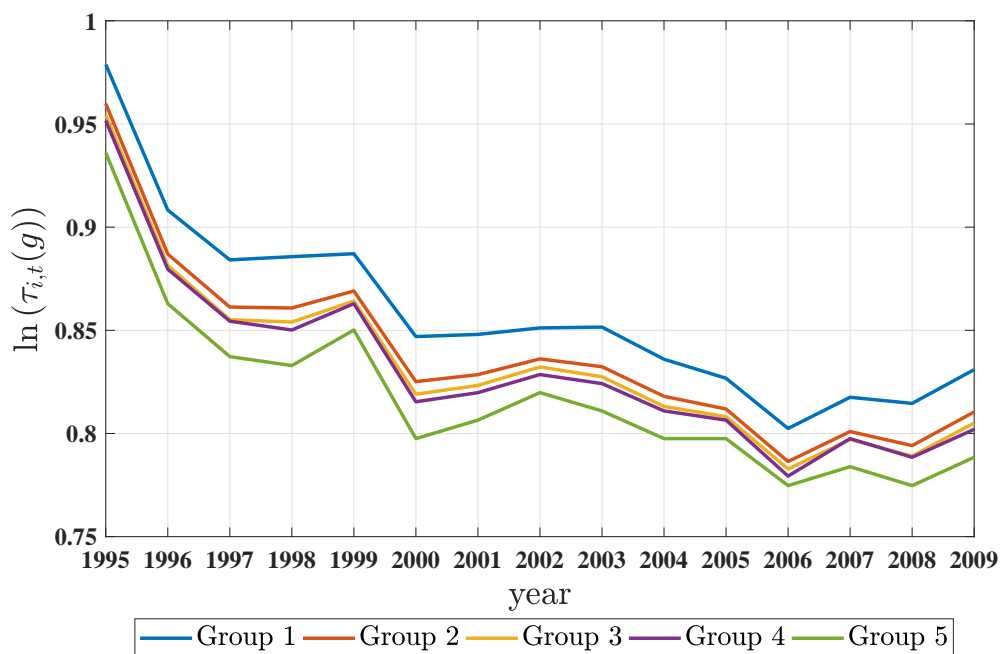
Fig. 24: Decomposition of Variable Trade Costs by Firm Size in Manufacturing
