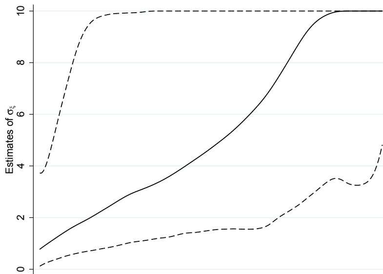
Figure 10: Physician-level estimates and bootstrapped 95% confidence intervals for \sigma_{\xi} . To ensure anonymity, the figure is LOWESS-smoothed with bandwidth 0.2.
