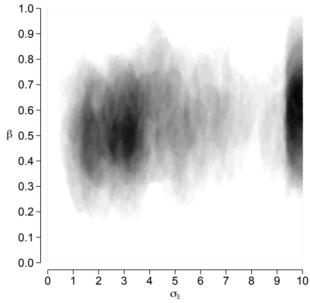
Figure 9: Heatmap of physician-level estimates for b and \sigma_\xi . To ensure anonymity, the figure shows a heatmap covering only areas of five physicians or more.
