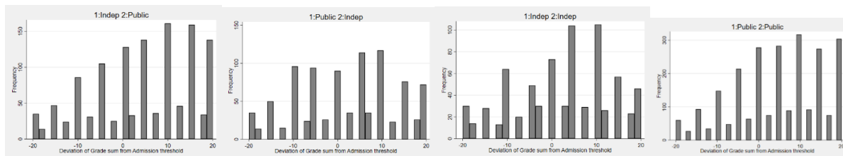
PANEL A: DATA WINDOW 20 UNITS AROUND THE ADMISSION THRESHOLDS
